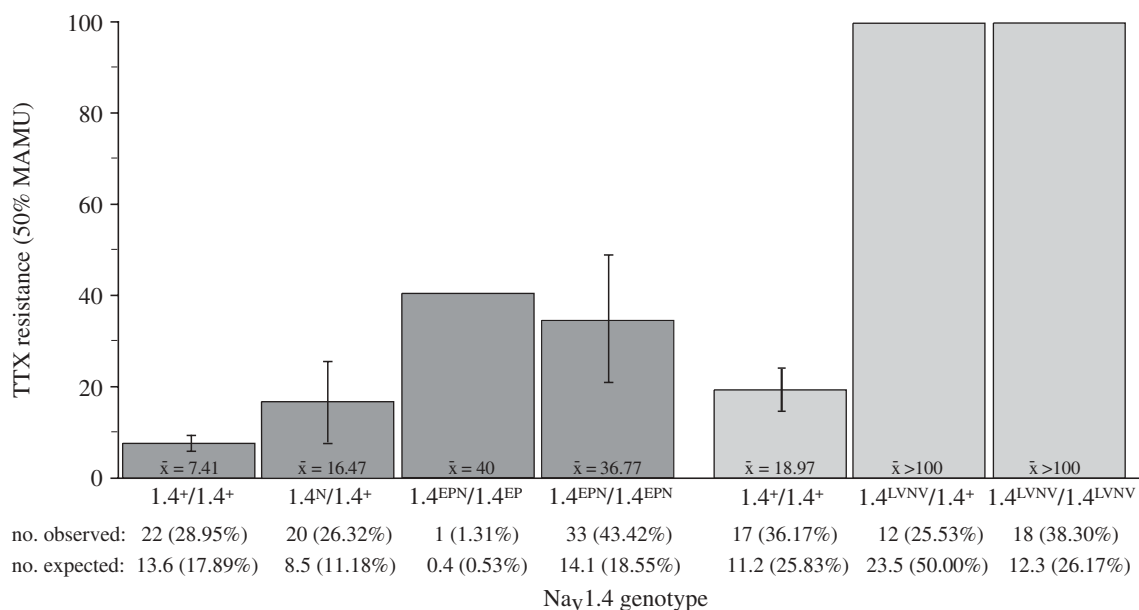
Figure 2. TTX resistance in T. atratus (dark grey) and T. sirtalis (light grey) allocated by Na v 1.4 genotype. For each genotype, mean TTX resistance, standard deviation (error bars), and observed versus expected genotypes are given. Note that some T. atratus genotypes were not detected in our sample (expected proportions do not total 100%). Due to the heightened resistance of T. sirtalis with derived Na v 1.4 alleles, we were forced to assign a minimum threshold value of TTX resistance and could not estimate phenotypic variance for these individuals (see text).
