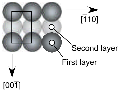
(c) fcc(110)
