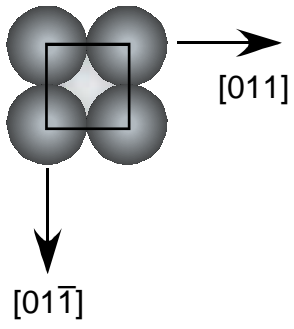
(a) fcc(100)
