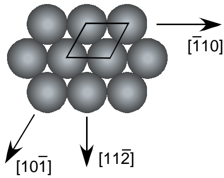
(b) fcc(111)
