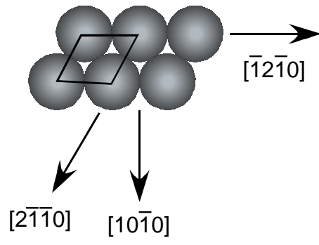
(a) hcp(0001) = (001)
