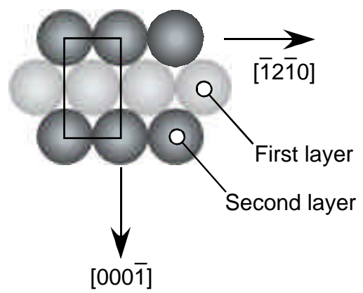
(b) hcp(10 \bar{1}0 ) = (100)
