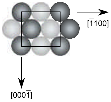
(c) hcp(11 \bar{2}0 ) = (110)
