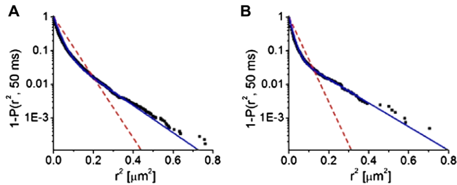
Fig. 2. Cumulative distribution functions derived from SPT data of tethered vesicles (A) and supported double membranes (B). Both systems contained single-molecule concentrations of Alexa647-labeled syntaxin-1A. From reconstructions of the particle trajectories, the cumulative distribution functions for the smallest time lag were generated. Fits to one-fraction diffusion are shown as red dashed lines, and fits to the two-fraction diffusion model are shown as solid blue lines. The best fit results and statistics are listed in Table 1.
