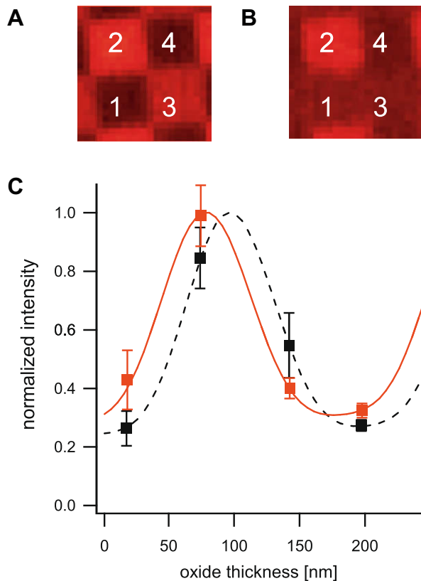
Fig. 3. FLIC measurements. (A) Fluorescence micrograph of Rh-DPPE-doped supported bilayer on 4-oxide FLIC chip. Numbers indicate the 4-oxide levels. Width of one square is 5 \mu\text{m} . (B) Fluorescence micrograph of Rh-DPPE-doped supported double membrane on 4-oxide FLIC chip. (C) FLIC data and fitted theory of supported bilayer (dashed black) and supported double membrane (solid red). Mean intensities and standard deviations of the fluorescence intensities were extracted from the 4-oxide levels in A and B. The supported bilayer data was fitted with a membrane-substrate distance of 1.7 \pm 0.7 nm. The supported double membrane was fitted with an inter-membrane distance of 14.6 \pm 2.0 nm.
